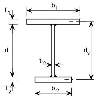
Figure 4.2 Warping and torsional constants for asymmetrical plate girders
