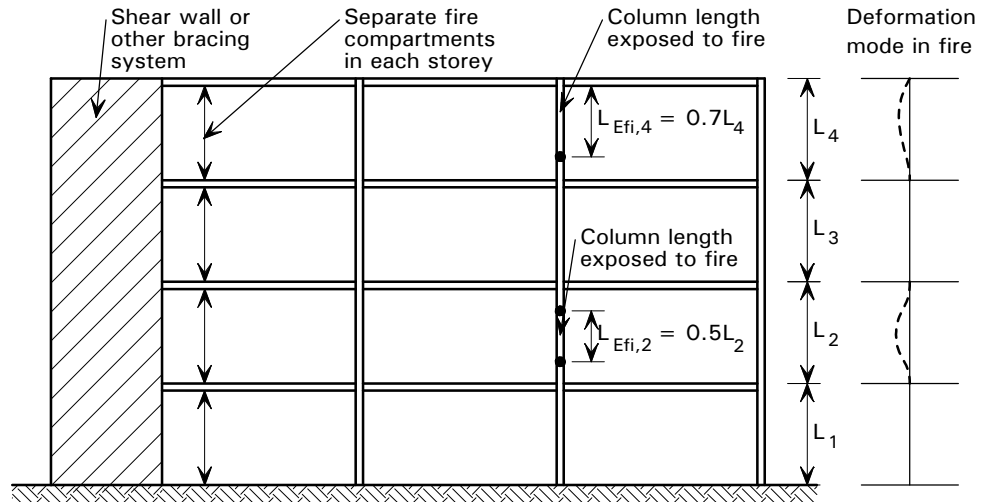
Figure 6.1 Buckling lengths L_{Efi} of columns in braced frames
