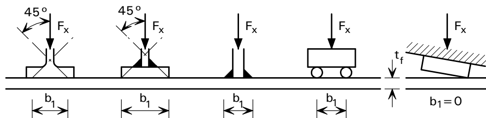
Figure 4.5 Length of stiff bearing, b_1
