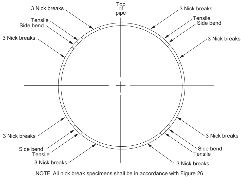
Figure 31—Location of Test Butt Weld Specimens for Flash Weld Procedure Qualification Test: Outside Diameter Greater Than 24 in. (610 mm) but Less Than or Equal to 30 in. (762 mm)
