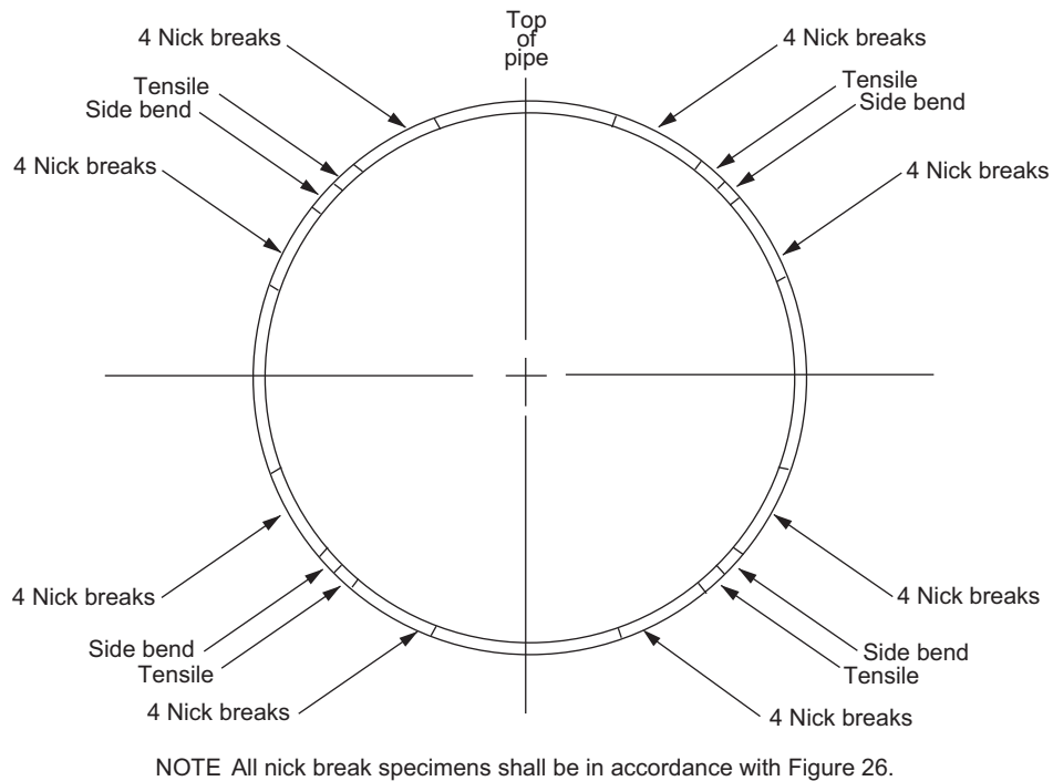
Figure 32—Location of Test Butt Weld Specimens for Flash Weld Procedure Qualification Test: Outside Diameter Greater Than 30 in. (762 mm)
